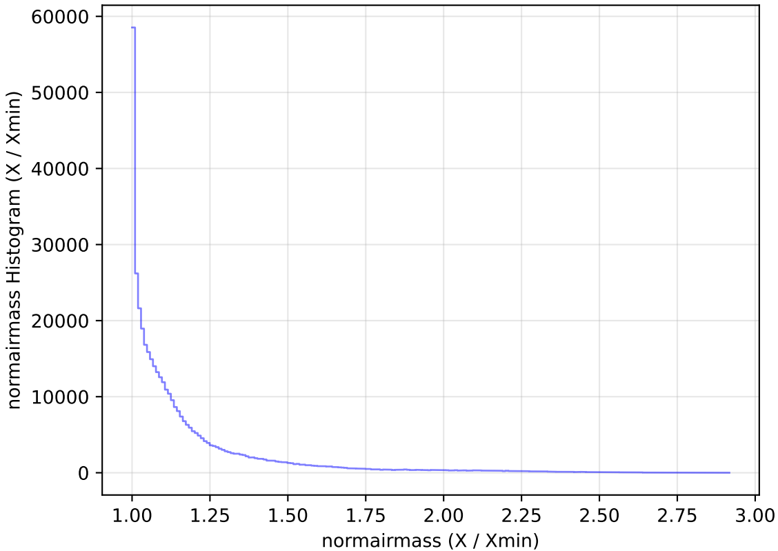
too_elab_r256_d2_gz_v3.4_10yrs WFD z band: normairmass Histogram
