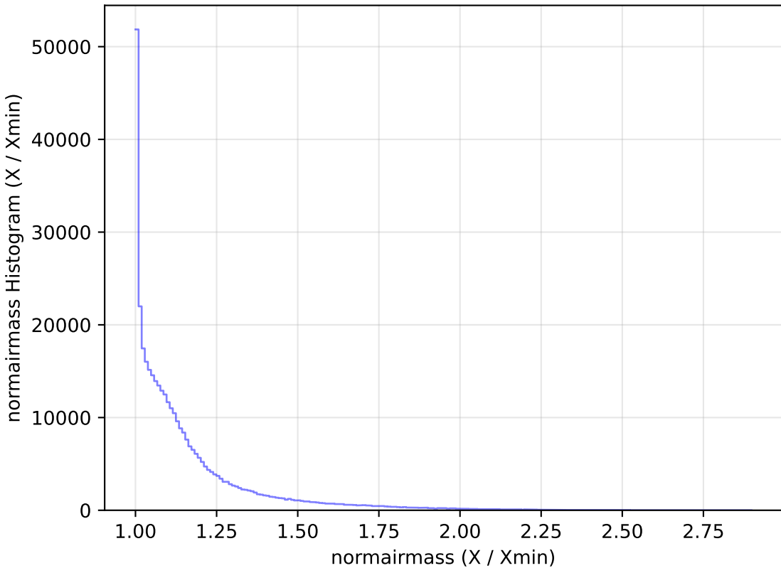
too_elab_r256_d2_gz_v3.4_10yrs WFD y band: normairmass Histogram
