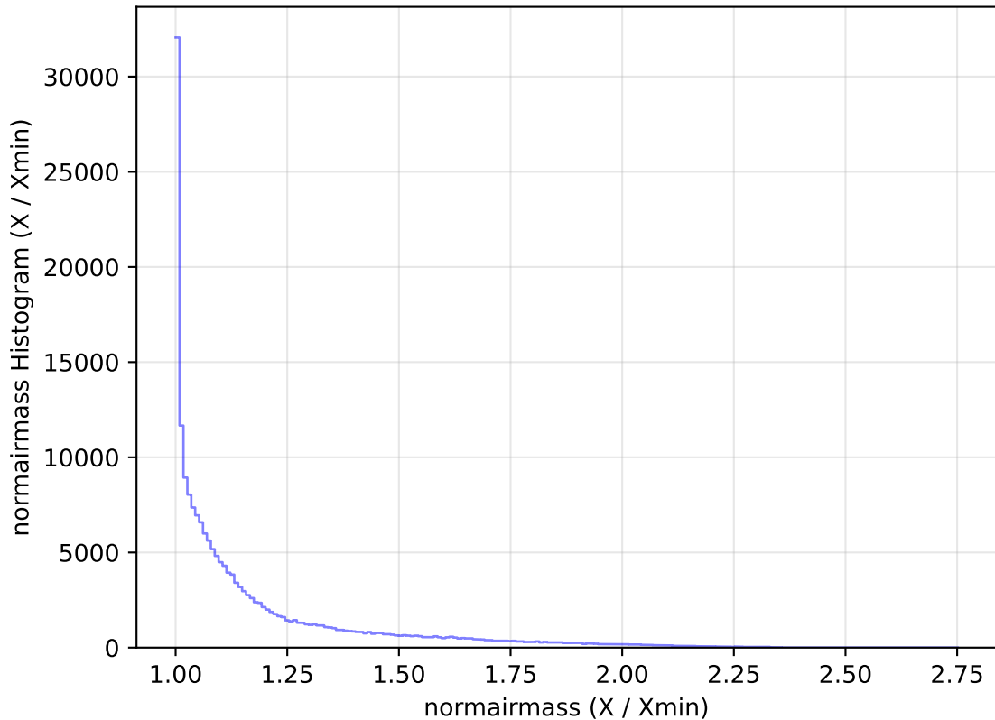
too_elab_r256_d2_gz_v3.4_10yrs WFD g band: normairmass Histogram
