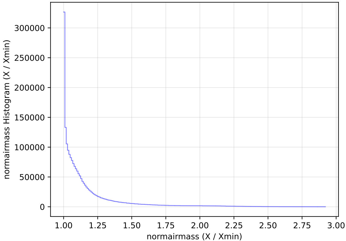
too_elab_r256_d2_gz_v3.4_10yrs WFD all bands: normairmass Histogram
