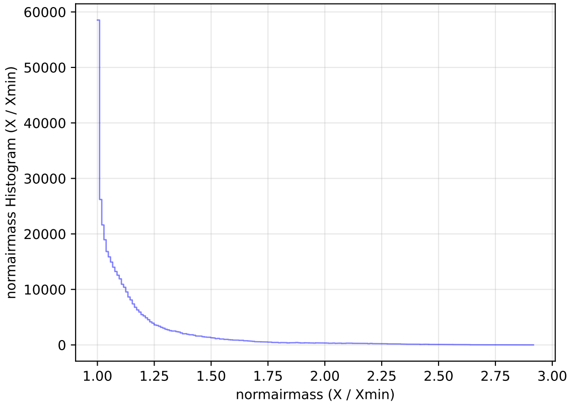
too_elab_r256_d2_gz_v3.4_10yrs All sky z band: normairmass Histogram
