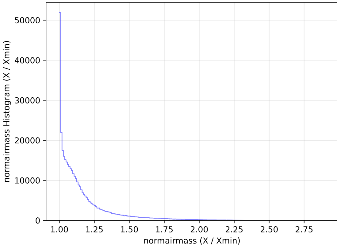
too_elab_r256_d2_gz_v3.4_10yrs All sky y band: normairmass Histogram
