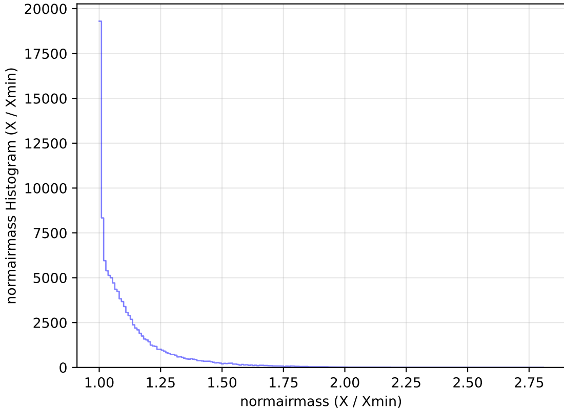
too_elab_r256_d2_gz_v3.4_10yrs All sky u band: normairmass Histogram
