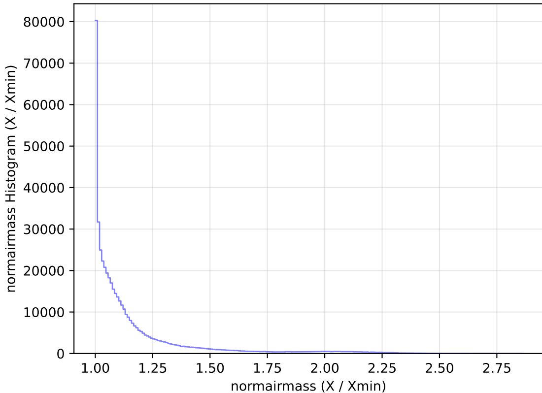
too_elab_r256_d2_gz_v3.4_10yrs All sky r band: normairmass Histogram
