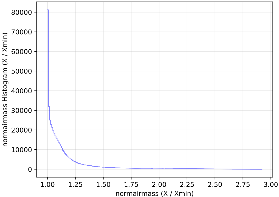
too_elab_r256_d2_gz_v3.4_10yrs All sky i band: normairmass Histogram
