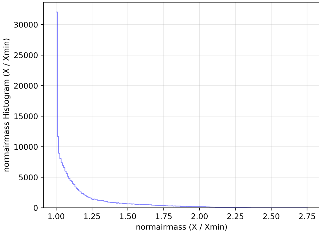
too_elab_r256_d2_gz_v3.4_10yrs All sky g band: normairmass Histogram
