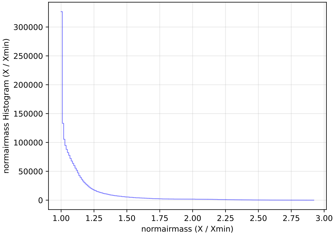
too_elab_r256_d2_gz_v3.4_10yrs All sky all bands: normairmass Histogram
