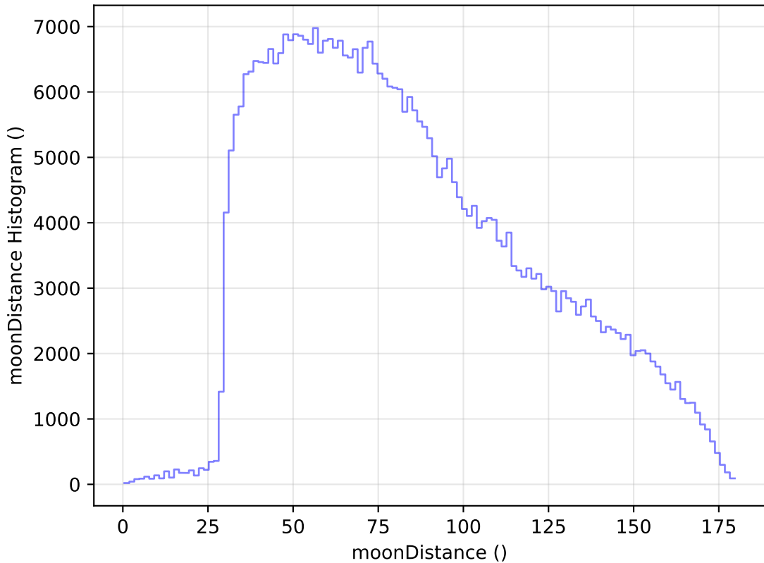
too_elab_r256_d2_gz_v3.4_10yrs WFD z band: moonDistance Histogram
