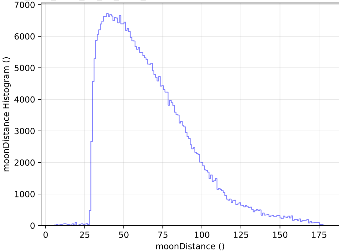
too_elab_r256_d2_gz_v3.4_10yrs WFD y band: moonDistance Histogram
