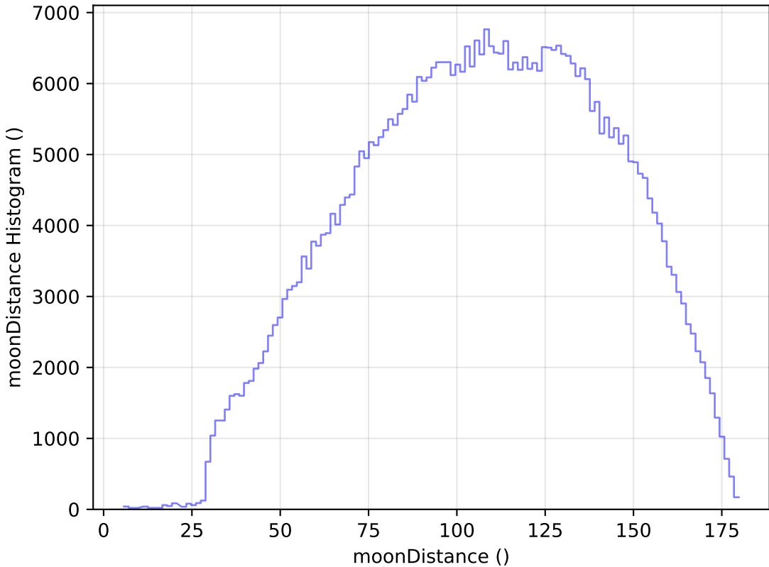
too_elab_r256_d2_gz_v3.4_10yrs WFD r band: moonDistance Histogram
