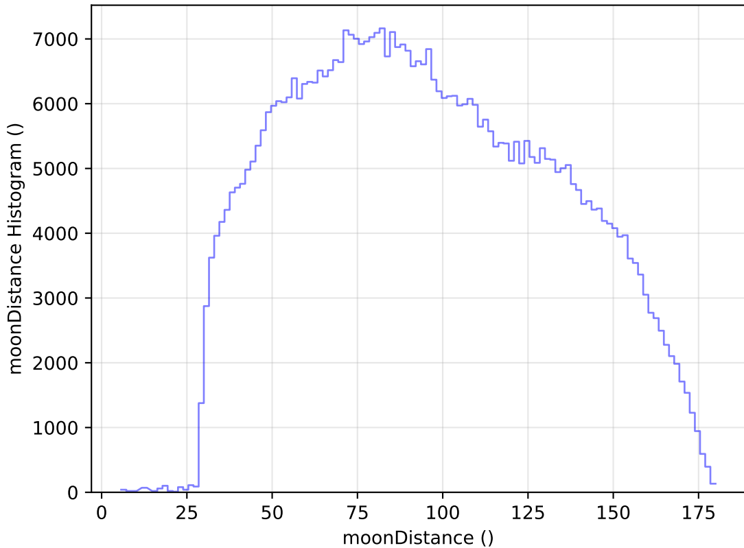
too_elab_r256_d2_gz_v3.4_10yrs WFD i band: moonDistance Histogram
