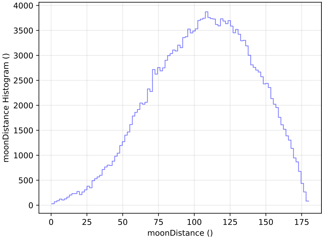
too_elab_r256_d2_gz_v3.4_10yrs WFD g band: moonDistance Histogram
