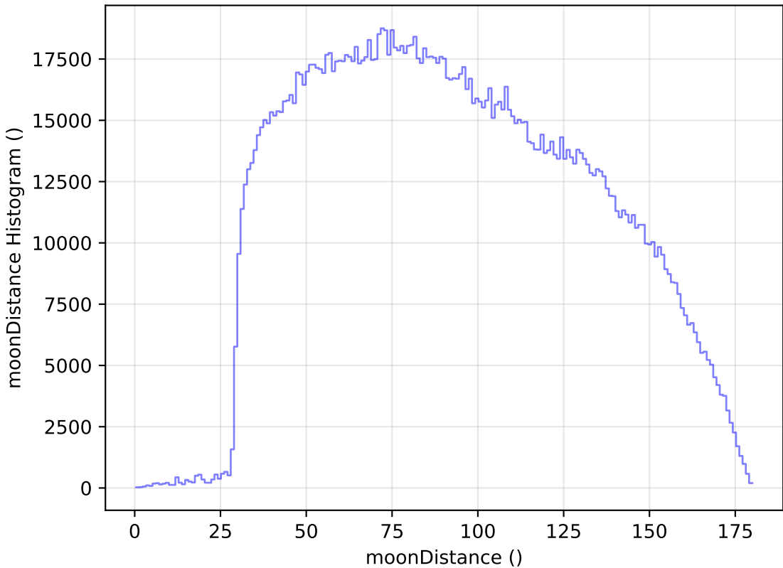
too_elab_r256_d2_gz_v3.4_10yrs WFD all bands: moonDistance Histogram
