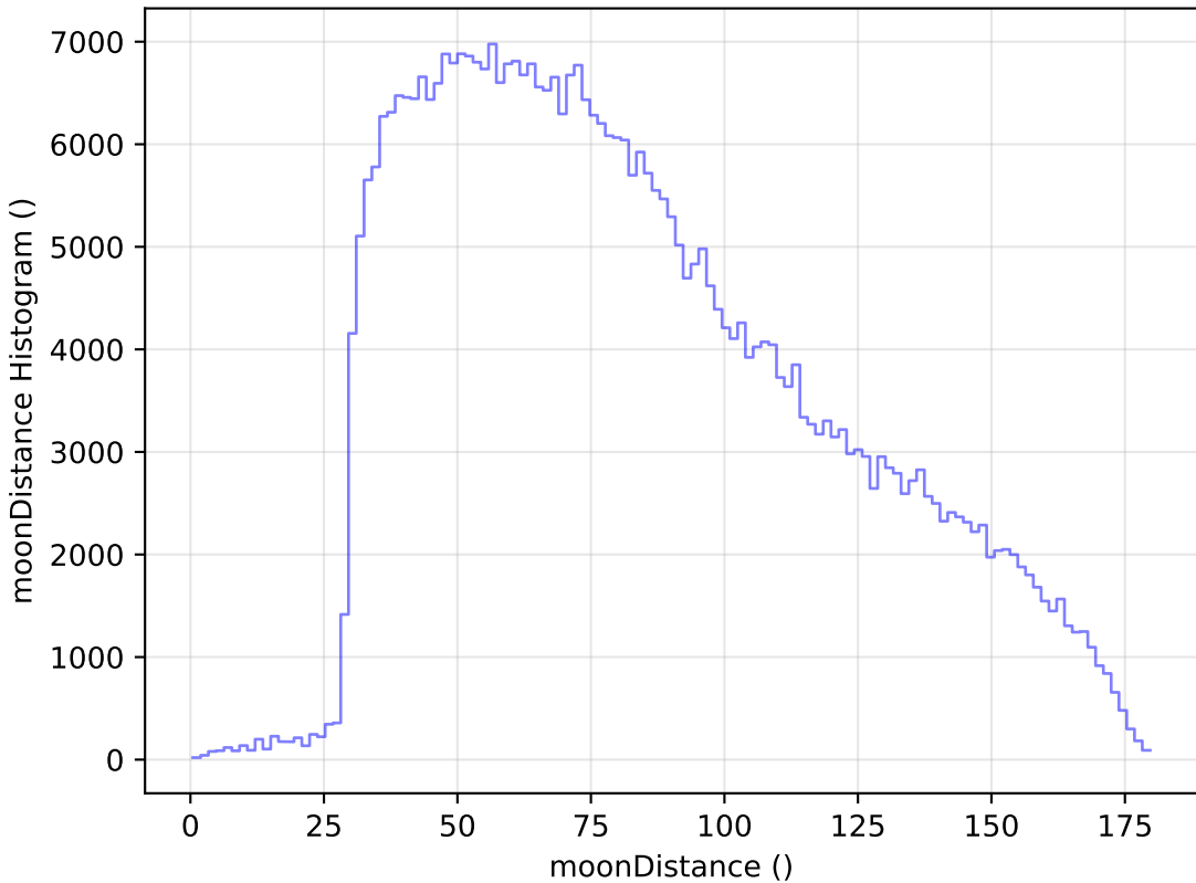
too_elab_r256_d2_gz_v3.4_10yrs All sky z band: moonDistance Histogram
