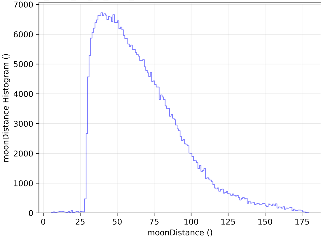
too_elab_r256_d2_gz_v3.4_10yrs All sky y band: moonDistance Histogram
