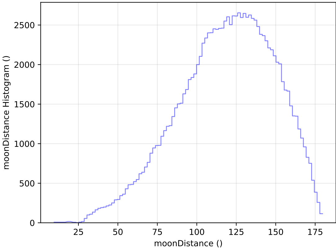
too_elab_r256_d2_gz_v3.4_10yrs All sky u band: moonDistance Histogram
