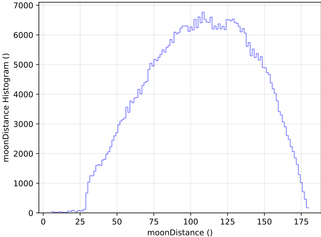
too_elab_r256_d2_gz_v3.4_10yrs All sky r band: moonDistance Histogram
