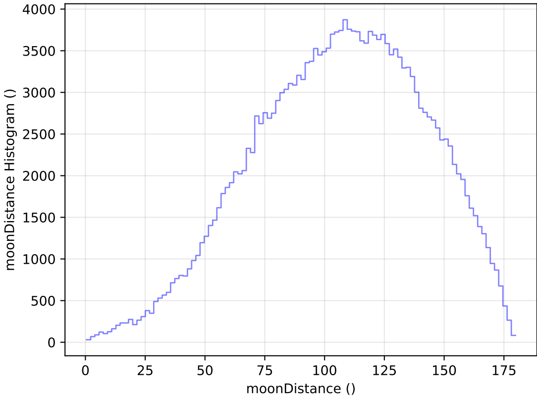
too_elab_r256_d2_gz_v3.4_10yrs All sky g band: moonDistance Histogram
