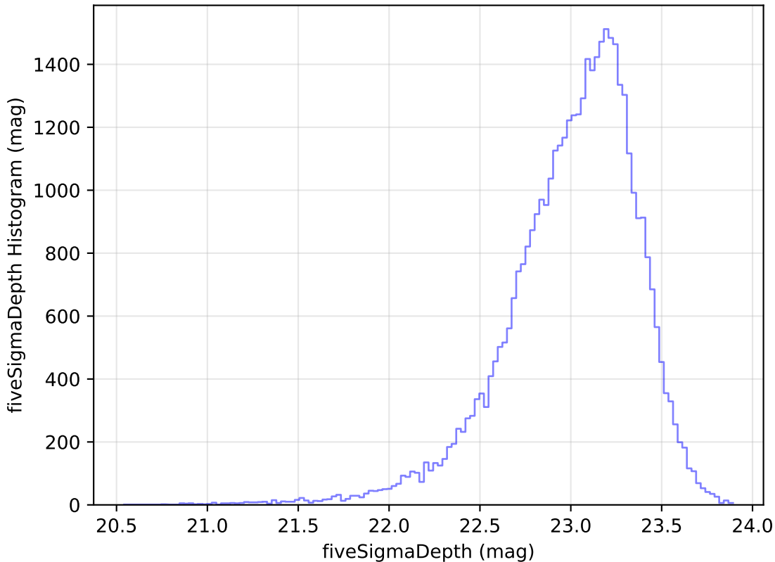
too_elab_r256_d2_gz_v3.4_10yrs Yr 1 z band: fiveSigmaDepth Histogram
