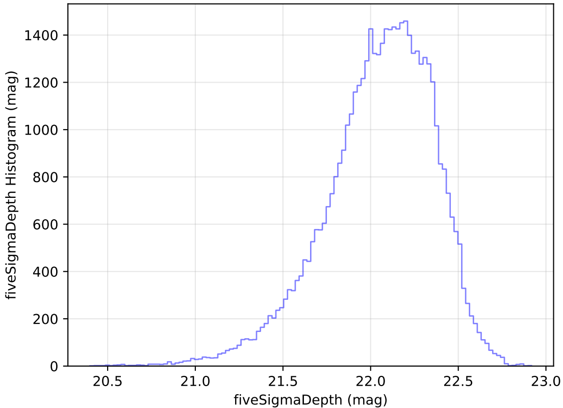
too_elab_r256_d2_gz_v3.4_10yrs Yr 1 y band: fiveSigmaDepth Histogram
