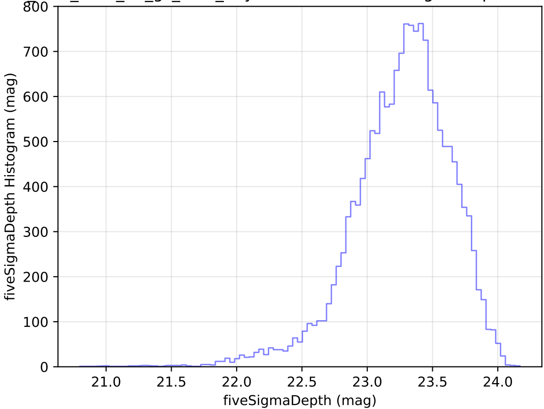
too_elab_r256_d2_gz_v3.4_10yrs Yr 1 u band: fiveSigmaDepth Histogram
