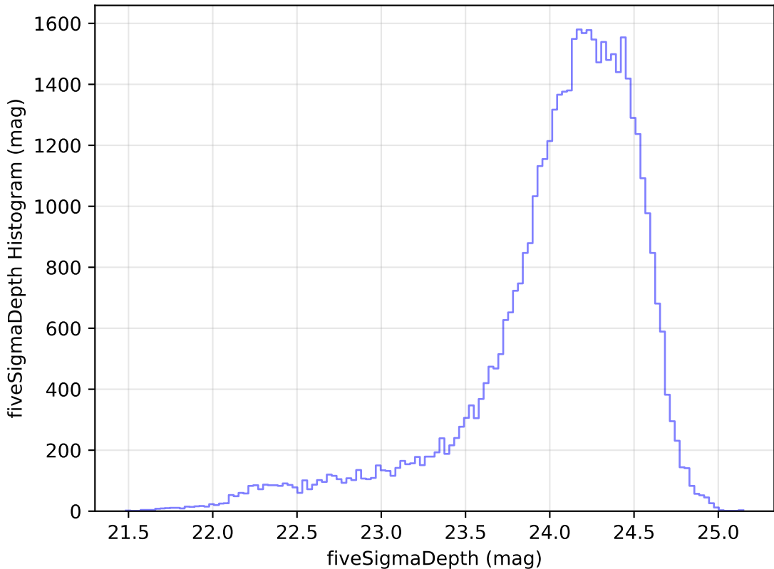
too_elab_r256_d2_gz_v3.4_10yrs Yr 1 r band: fiveSigmaDepth Histogram
