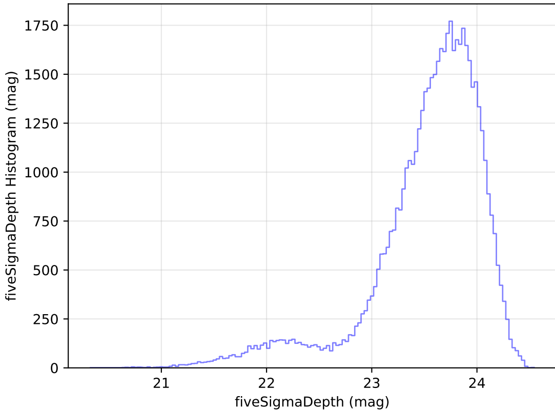
too_elab_r256_d2_gz_v3.4_10yrs Yr 1 i band: fiveSigmaDepth Histogram
