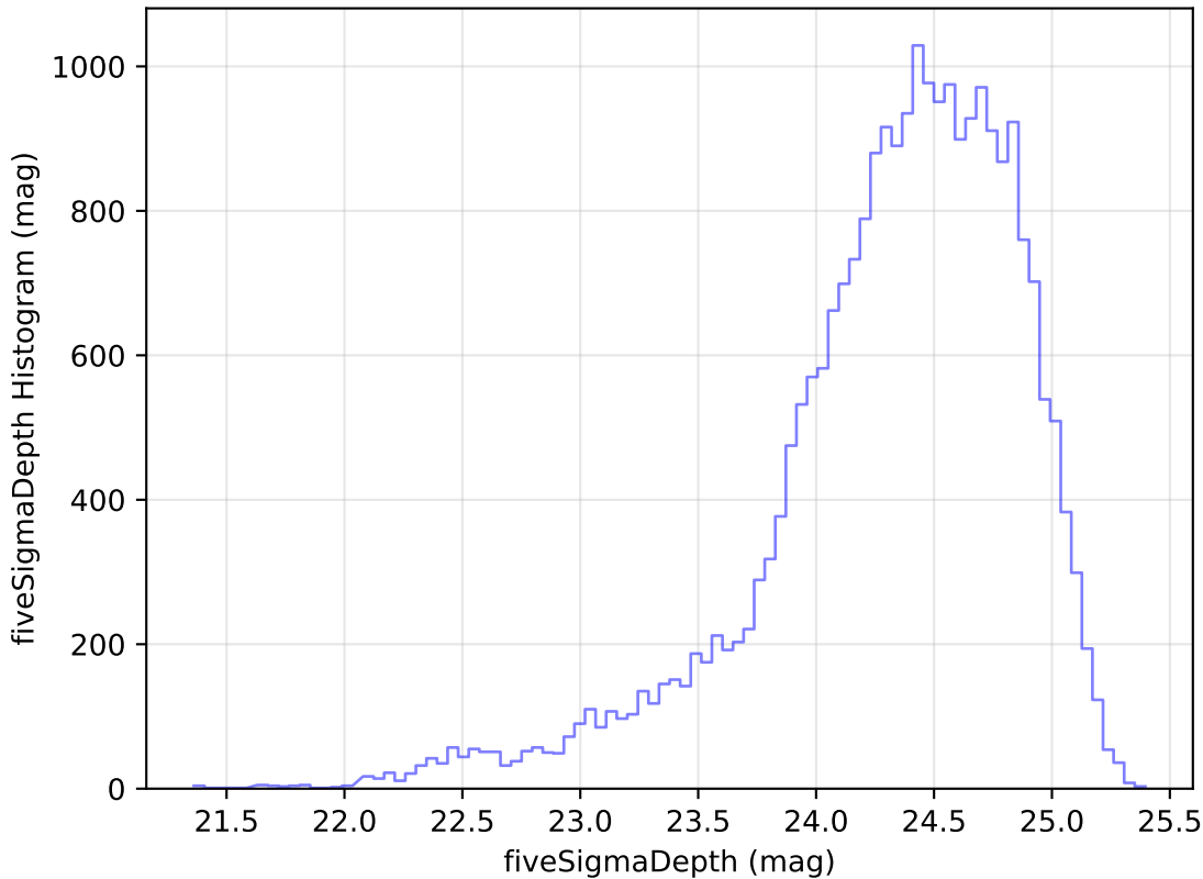
too_elab_r256_d2_gz_v3.4_10yrs Yr 1 g band: fiveSigmaDepth Histogram
