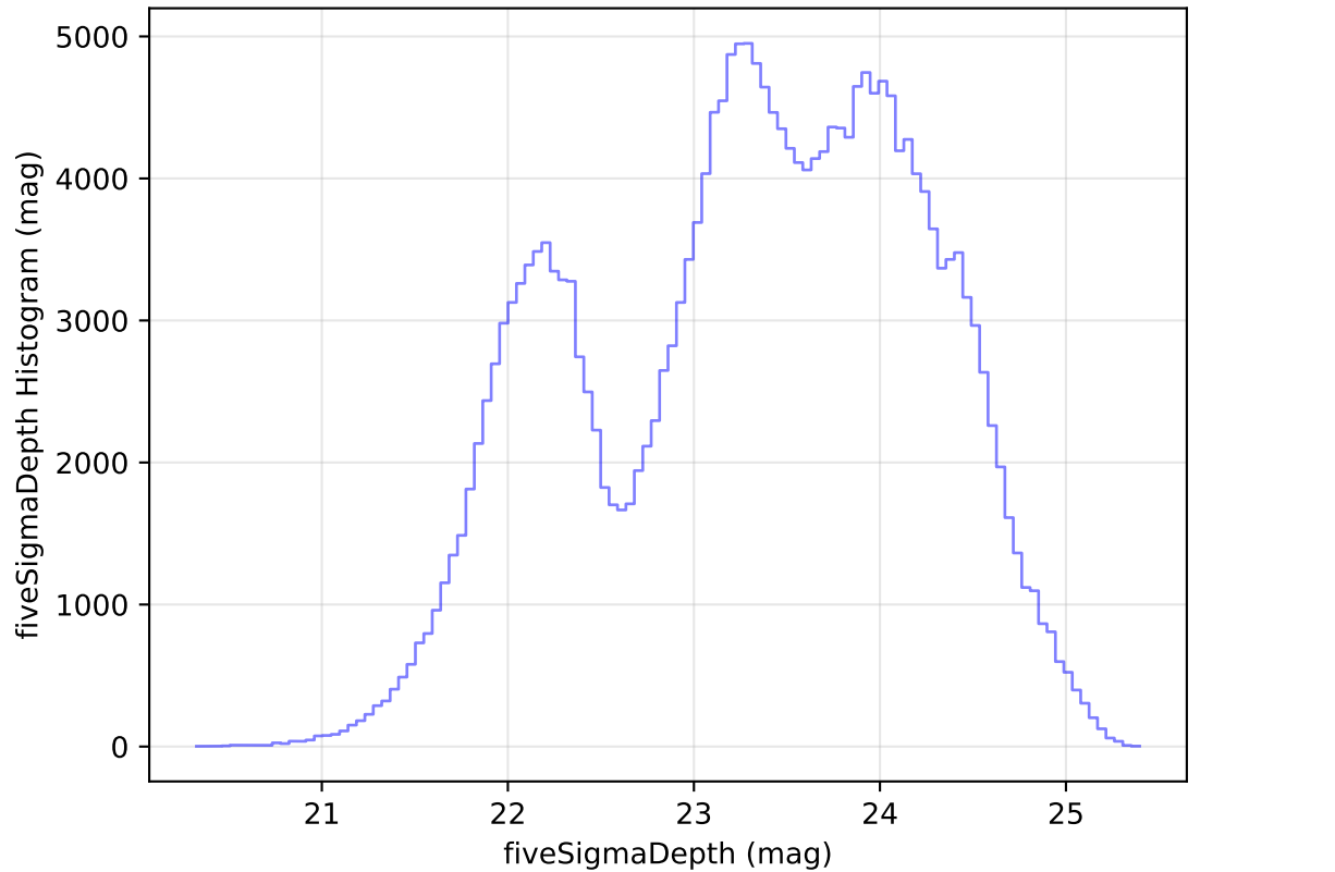
too_elab_r256_d2_gz_v3.4_10yrs Yr 1 all bands: fiveSigmaDepth Histogram
