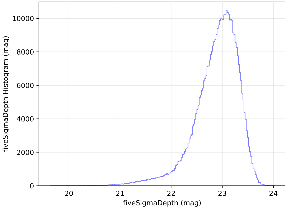
too_elab_r256_d2_gz_v3.4_10yrs WFD z band: fiveSigmaDepth Histogram
