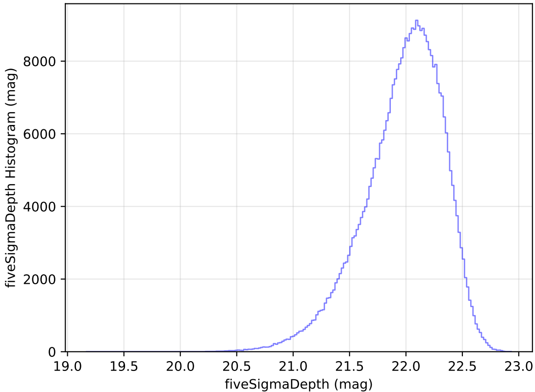
too_elab_r256_d2_gz_v3.4_10yrs WFD y band: fiveSigmaDepth Histogram
