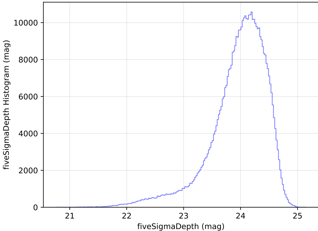
too_elab_r256_d2_gz_v3.4_10yrs WFD r band: fiveSigmaDepth Histogram
