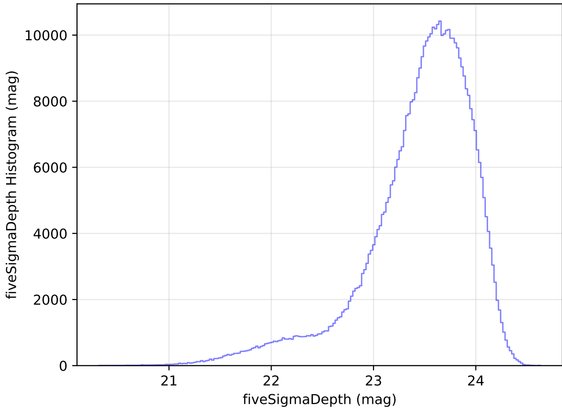
too_elab_r256_d2_gz_v3.4_10yrs WFD i band: fiveSigmaDepth Histogram
