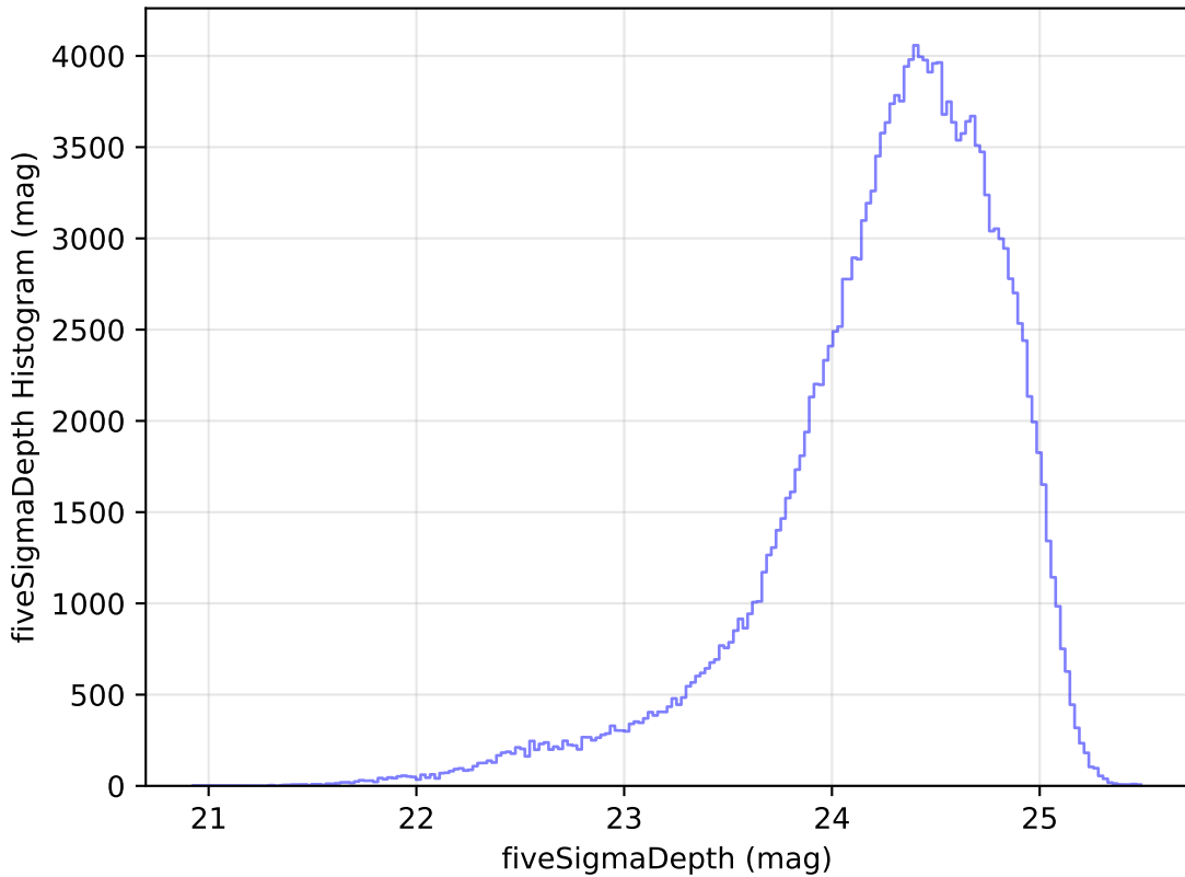
too_elab_r256_d2_gz_v3.4_10yrs WFD g band: fiveSigmaDepth Histogram
