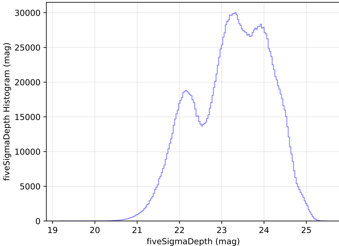
too_elab_r256_d2_gz_v3.4_10yrs WFD all bands: fiveSigmaDepth Histogram
