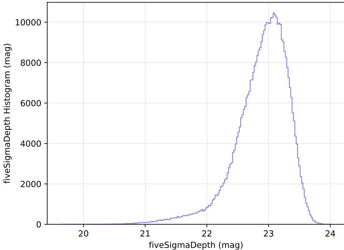
too_elab_r256_d2_gz_v3.4_10yrs All sky z band: fiveSigmaDepth Histogram
