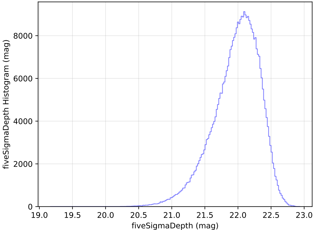
too_elab_r256_d2_gz_v3.4_10yrs All sky y band: fiveSigmaDepth Histogram
