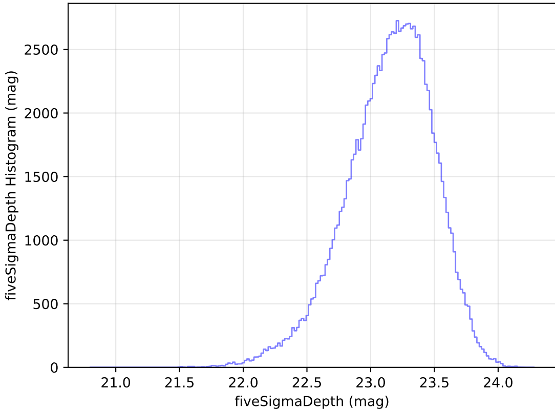
too_elab_r256_d2_gz_v3.4_10yrs All sky u band: fiveSigmaDepth Histogram
