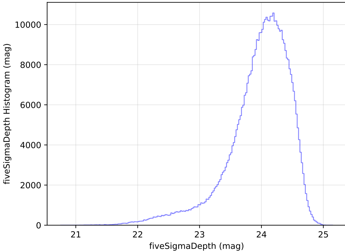
too_elab_r256_d2_gz_v3.4_10yrs All sky r band: fiveSigmaDepth Histogram
