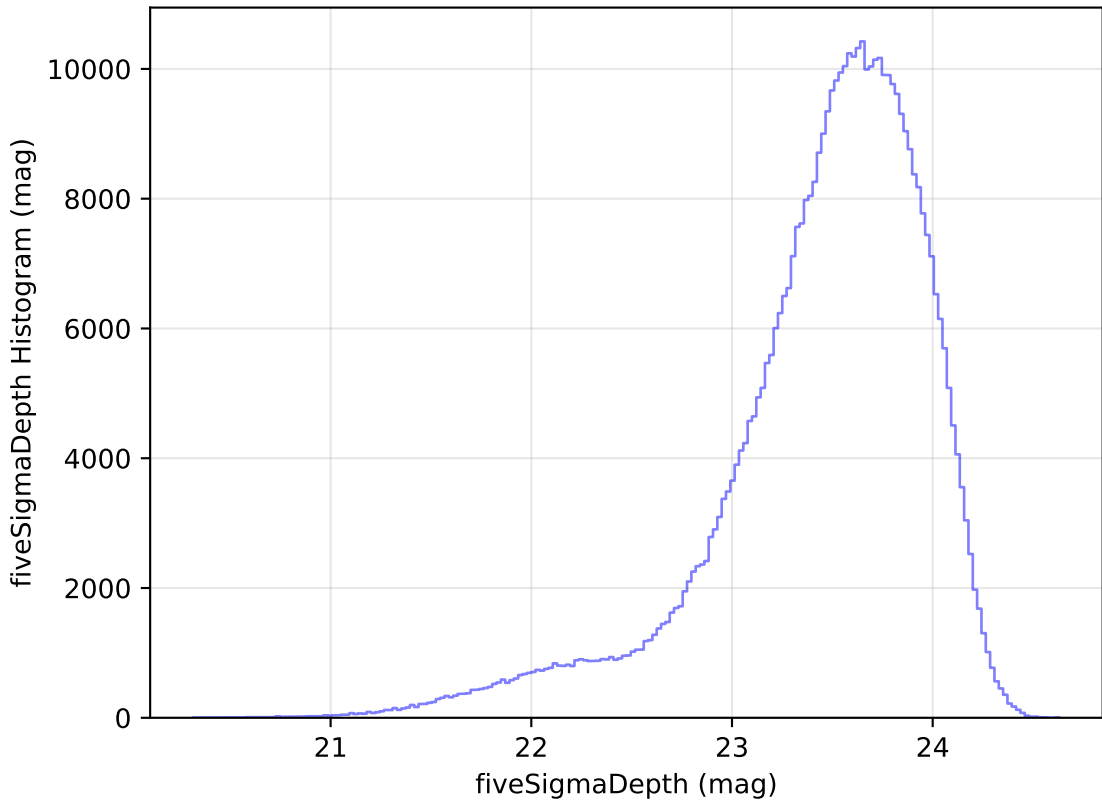
too_elab_r256_d2_gz_v3.4_10yrs All sky i band: fiveSigmaDepth Histogram
