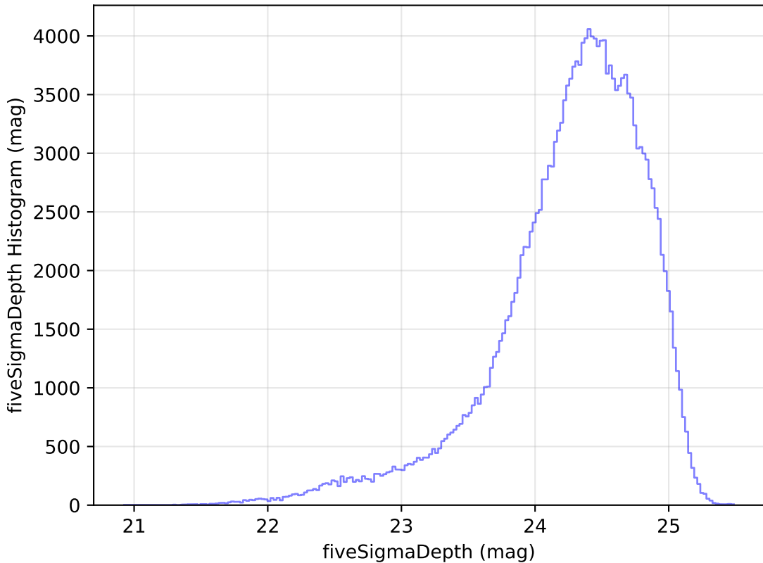
too_elab_r256_d2_gz_v3.4_10yrs All sky g band: fiveSigmaDepth Histogram
