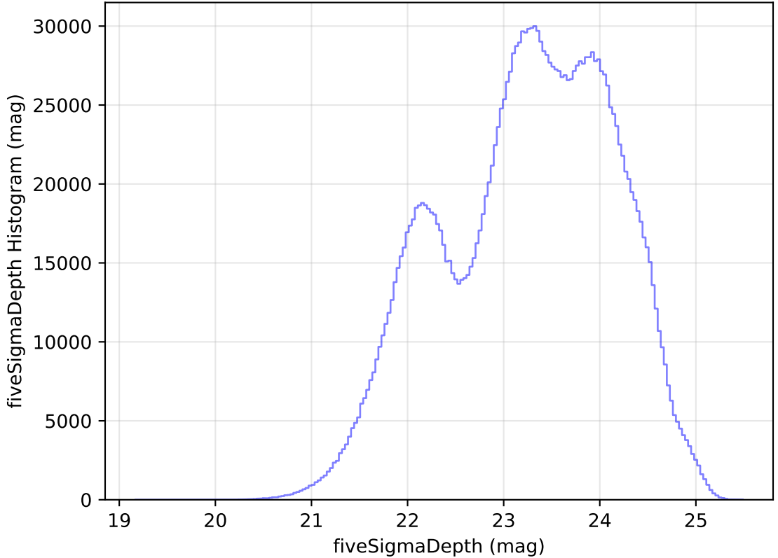
too_elab_r256_d2_gz_v3.4_10yrs All sky all bands: fiveSigmaDepth Histogram
