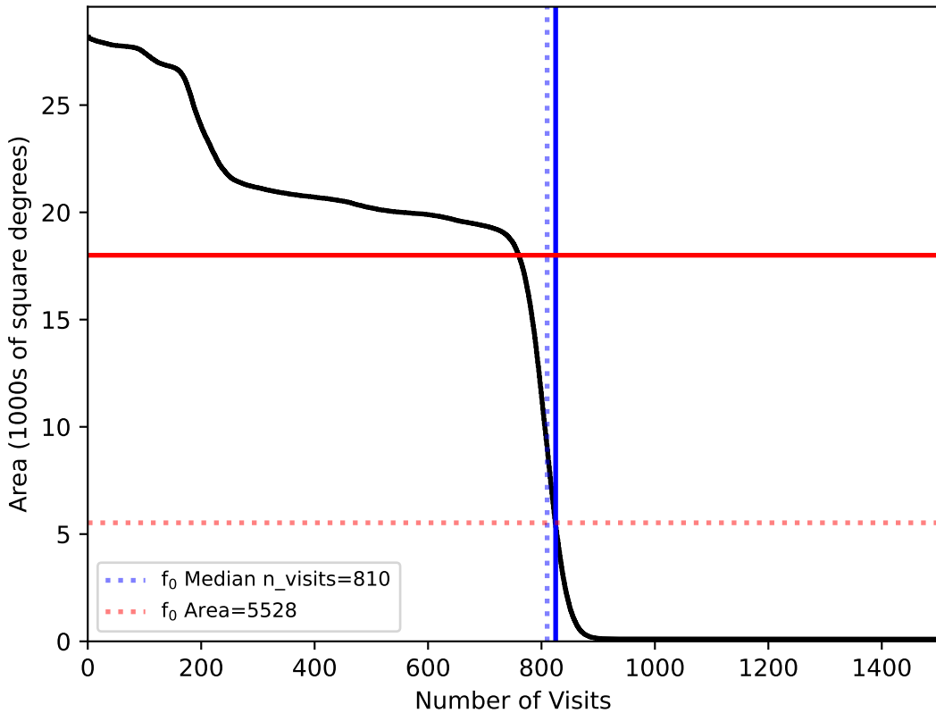
too_elab_r256_d2_gz_v3.4_10yrs All sky: fO
