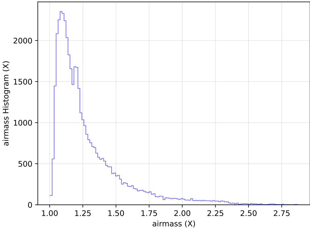
too_elab_r256_d2_gz_v3.4_10yrs Yr 1 z band: airmass Histogram
