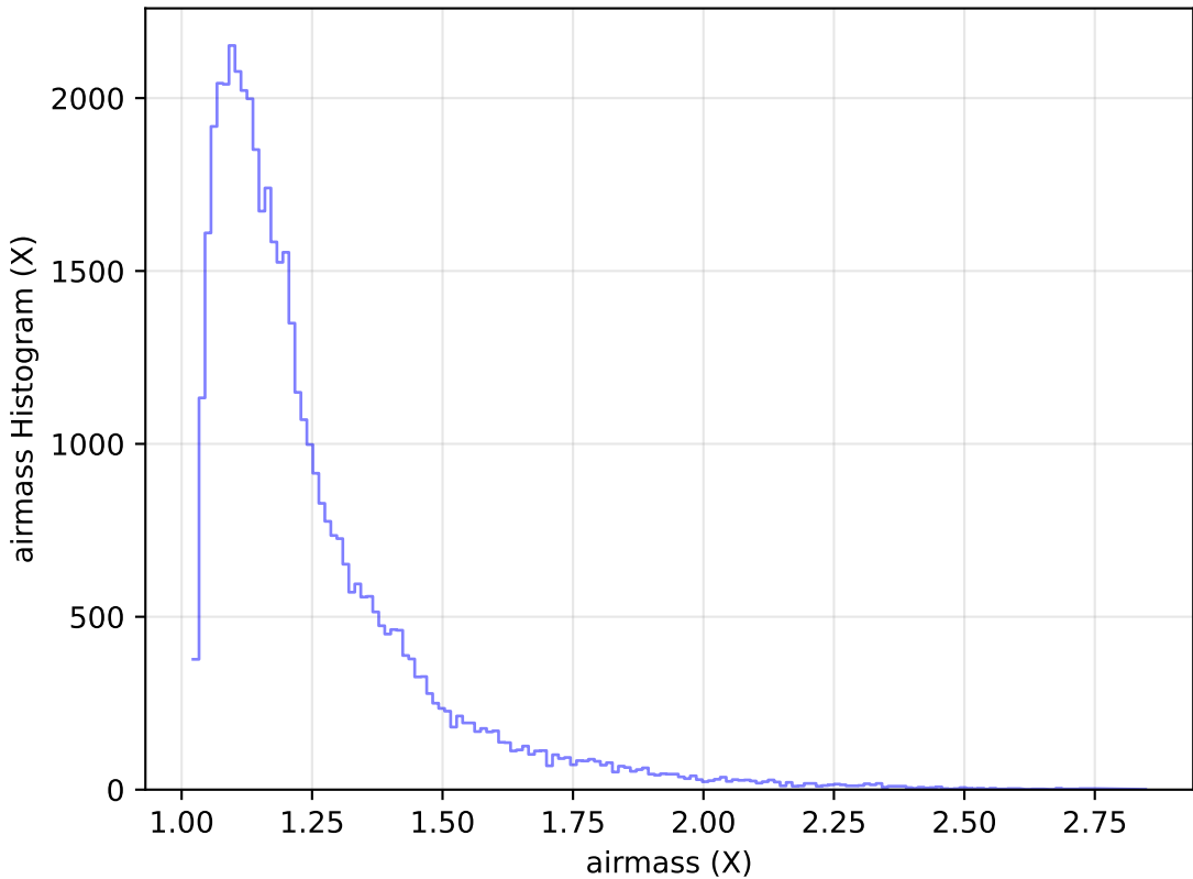
too_elab_r256_d2_gz_v3.4_10yrs Yr 1 y band: airmass Histogram
