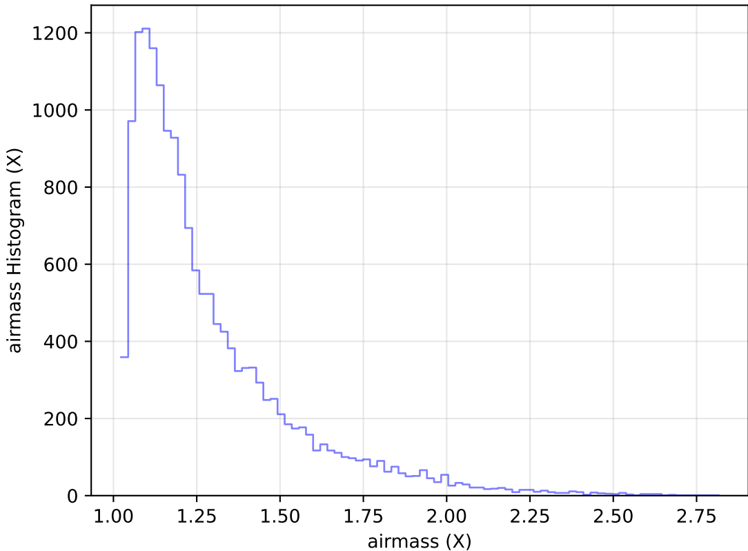
too_elab_r256_d2_gz_v3.4_10yrs Yr 1 u band: airmass Histogram
