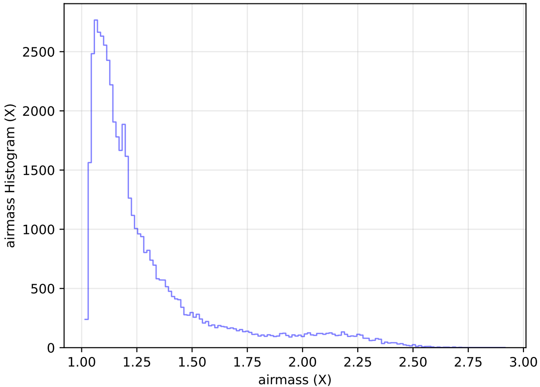
too_elab_r256_d2_gz_v3.4_10yrs Yr 1 r band: airmass Histogram
