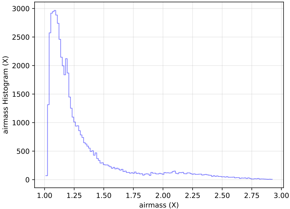
too_elab_r256_d2_gz_v3.4_10yrs Yr 1 i band: airmass Histogram
