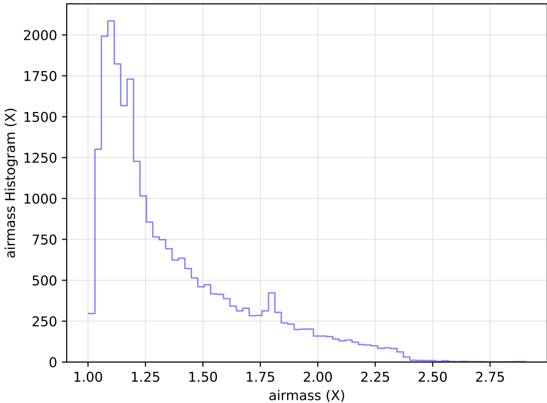
too_elab_r256_d2_gz_v3.4_10yrs Yr 1 g band: airmass Histogram
