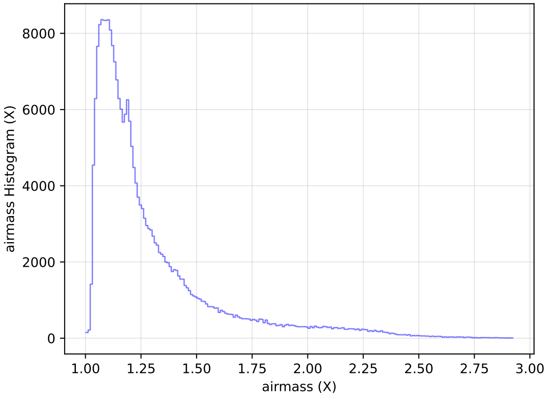
too_elab_r256_d2_gz_v3.4_10yrs Yr 1 all bands: airmass Histogram
